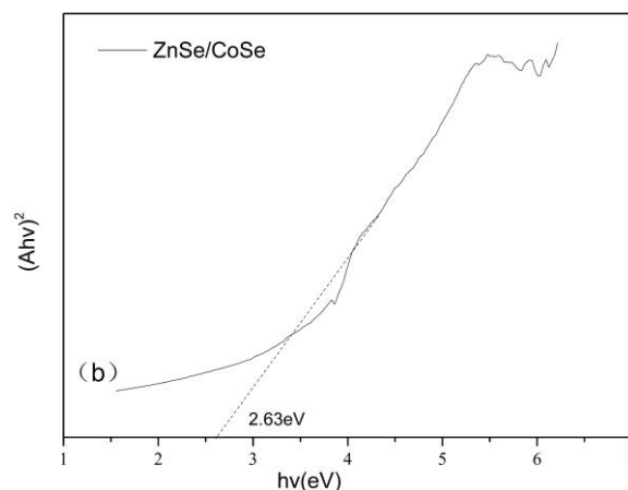
Fig. 4: UV-Vis absorption spectra (a) and estimated band gaps (b) of ZnSe/CoSe.
